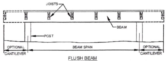
TYPICAL DECK BEAM SPANS
